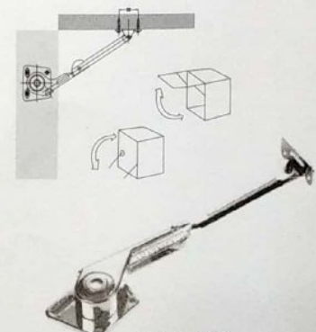
PFF-162 Soft Down Stay
