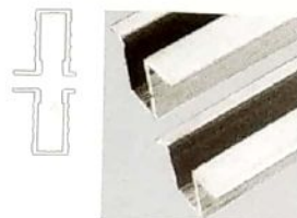
PSC-103 Size 3mtr. / 3.962 mtr. Max. Door weight 40kgs
